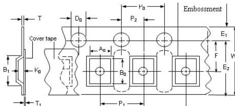
EIA Tape Component Dimensions
