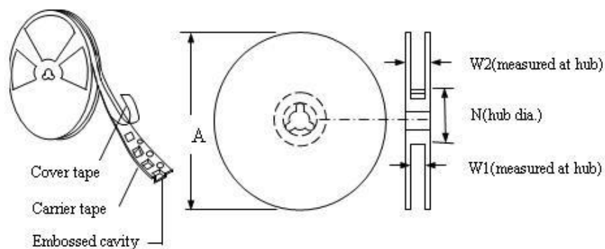
EIA Reel Dimensions
