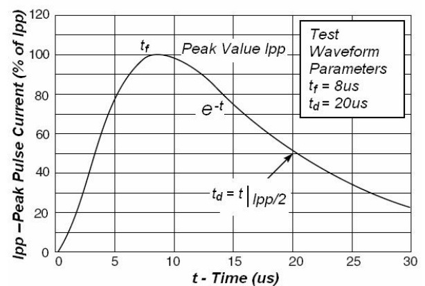
Figure 2- Pulse Waveform
